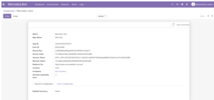
3basic_setup
