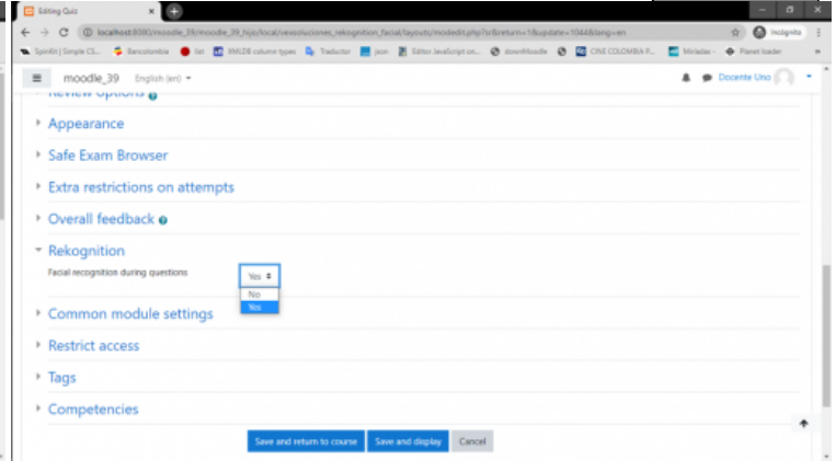
vexsoluciones_facial_recognition_config_quiz2
