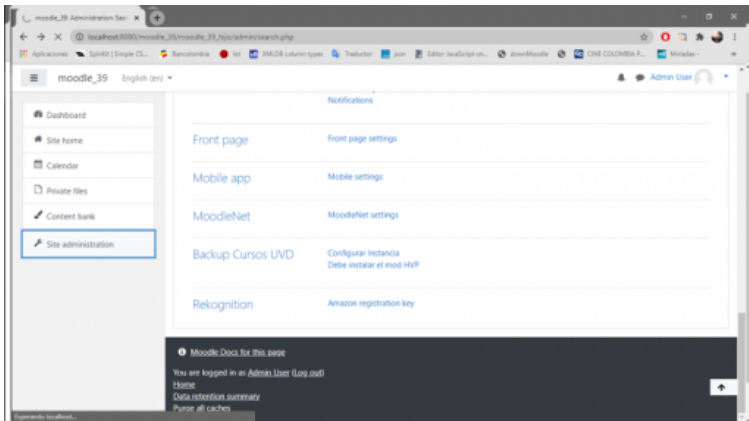
vexsoluciones_facial_recognition_config_key_edit2
